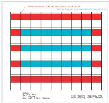
Polar Racking 10 Kw System Layout
