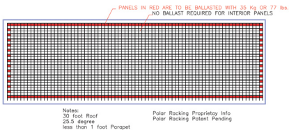
Polar Racking 250 Kw System Layout
